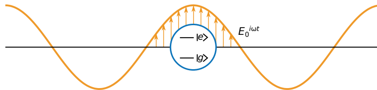
Figure 3.19: Sketch illustrating the semi-classical approach for describing an emitter exposed to a light field. The emitter is represented by a quantum mechanical two-level system with ground state |g\rangle and excited state |e\rangle . The light field is described by a classical electric field.
