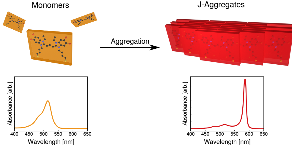
Figure 3.12: Schematic representation of the aggregation of TDBC monomers to J-aggregates. TDBC molecules are flat quasi two dimensional plates that form a brick like structure under aggregation. The spectrum of the J-aggregates exhibits a very sharp red-shifted peak that is not visible in pure monomer spectra.
