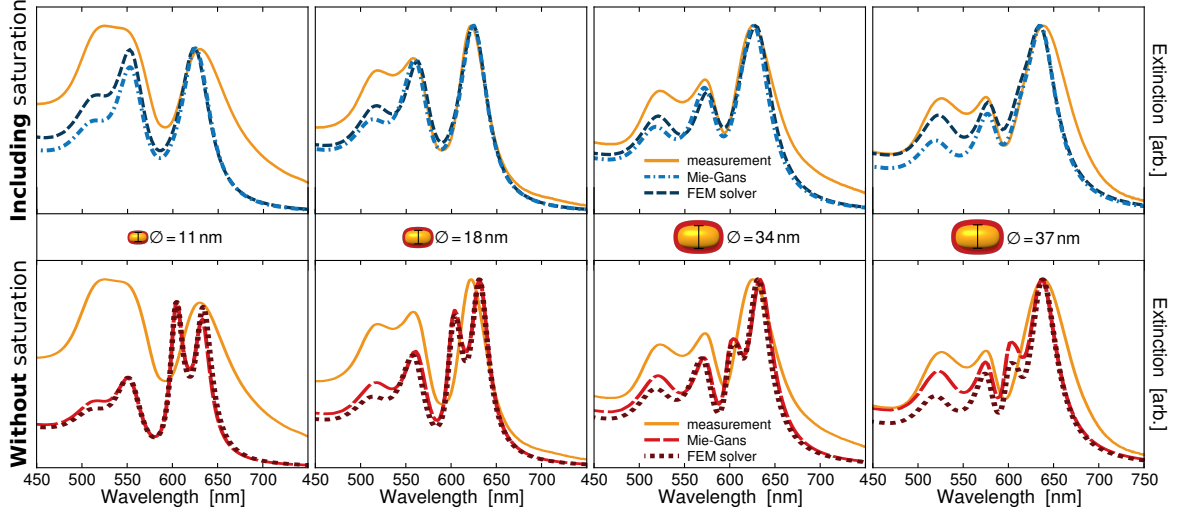
FIG. 3. The upper row shows the extinction spectra of TDBC-coated gold nanorods of different sizes as measured (orange solid lines) and simulated with to the Mie-Gans model (dash-dotted blue lines) and FEM (dashed dark blue lines). Both models include VISA. All particles have the same aspect ratio but a varying transverse diameter of 11 nm, 18 nm, 34 nm, and 37 nm (from left to right). The simulations included VISA. The lower row presents the same measured spectra (orange lines) with Mie-Gans-simulated (dashed red lines) and FEM-simulated (dotted dark red lines) that did not include saturation.
