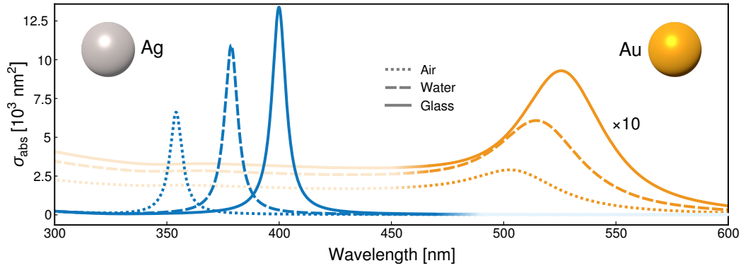
Figure 3.5: Absorption cross sections of silver (blue lines) and gold (red lines) nanospheres with a diameter of 25 nm in different media. The permittivities are chosen to be \epsilon_{\text{med}} = 1 (air, dotted lines), \epsilon_{\text{med}} = 1.7 (water, dashed lines) and \epsilon_{\text{med}} = 2.3 (glass, solid lines). The data for the permittivities of gold and silver were taken from Reference 37.
