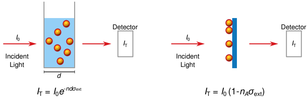
Figure 4.21: Scheme of transmission spectroscopy of nanoparticles in solution or on substrate. In both cases an incident beam with known intensity I_0 is guided through the samples and recorded by a detector. The transmitted light intensity is determined by Equations 4.1 and 4.3, respectively. The extinction cross section can then directly be retrieved.
