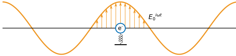
Figure 3.18: Sketch of the classical analogon to a two-level emitter exposed to light. An electron is described as oscillator bound to a rest position leading to a resonance frequency \omega_0 . The electron can oscillate in the classical electric light field.
