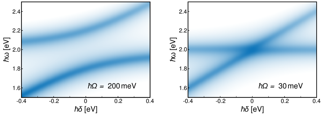
Figure 3.26: Amplitudes of two coupled oscillators damped by \hbar\gamma = 60\text{ meV} . The resonance of oscillator B is kept constant at \hbar\omega_B = 2\text{ eV} while the resonance of oscillator A is tuned. The plots are found by assuming the coupled modes to be Lorentz peaks with complex resonances \omega_{\pm} . The left panel depicts the situation with \hbar\Omega = 200\text{ meV} , the right panel that with \hbar\Omega = 30\text{ meV} . While on the left side, a clear anticrossing is visible the branches seem to cross in the right panel.
