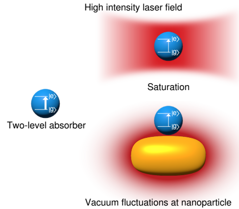
FIG. 1. Sketch of the phenomenon. A two-level absorber is saturated by high intensities. These can be reached by a high intensity laser or by the vacuum field fluctuations in ultrasmall cavities.
