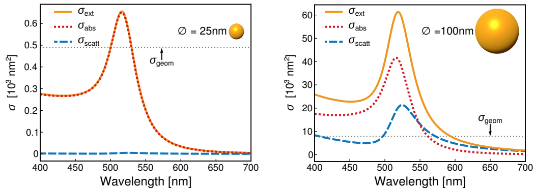
Figure 3.6: Scattering (dashed blue line), absorption (dotted red line) and extinction (orange solid line) cross sections of gold nano spheres with a diameter of 25 nm in the left panel and 100 nm on the right side. For small particles, scattering can be neglected and absorption completely dominates the extinction. For larger particles, scattering becomes more relevant and notably contributes to the extinction, as well. As comparison, the dotted grey lines mark the geometrical cross sections of the two particles. The data for the permittivities of gold and silver were taken from Reference 37.
