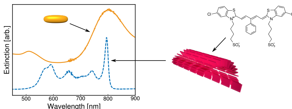
Figure 4.6: Gold nanorods and J-aggregates with resonances in the infrared. The right side depicts the chemical structure of S 2284 and the tubular structure of its J-aggregate. The respective extinction spectrum is presented in the left panel by the dashed blue line exhibiting a sharp J-aggregate peak around 800 nm. The panel also shows the extinction of gold nanorods with a nominal transverse resonance at 800 nm as orange line. The spectra are shifted by an offset for clarity.
