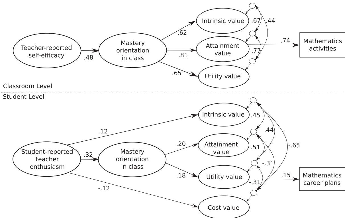
Fig. 1. Empirical multilevel structural equation model for the examined relations. Only significant ( p < 0.05 ) standardized coefficients are depicted.
