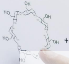
\beta -Cyclodextrin (0.07 mmol)
